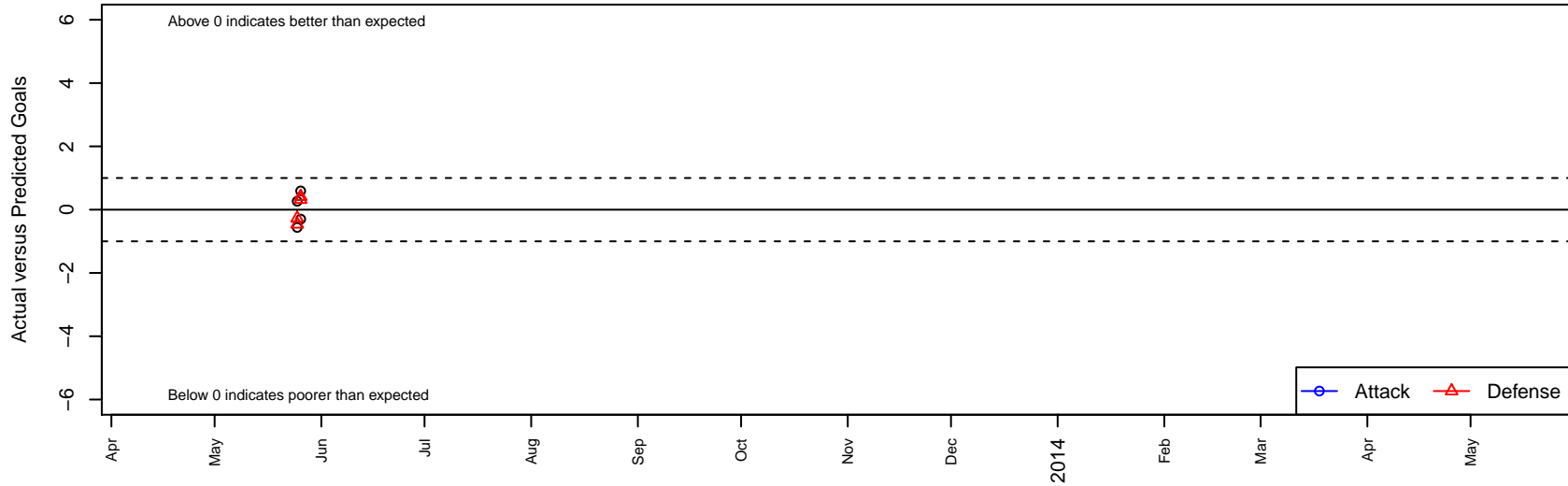
RVSC Timbers Fuego B94 Dots are actual minus expected GF (blue circles) and GA (red triangles). Blue line is smoothed change in attack strength. Red is smoothed change in defense strength.
